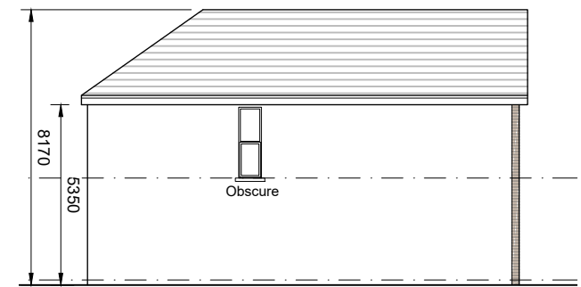
Side Elevation 1:200
